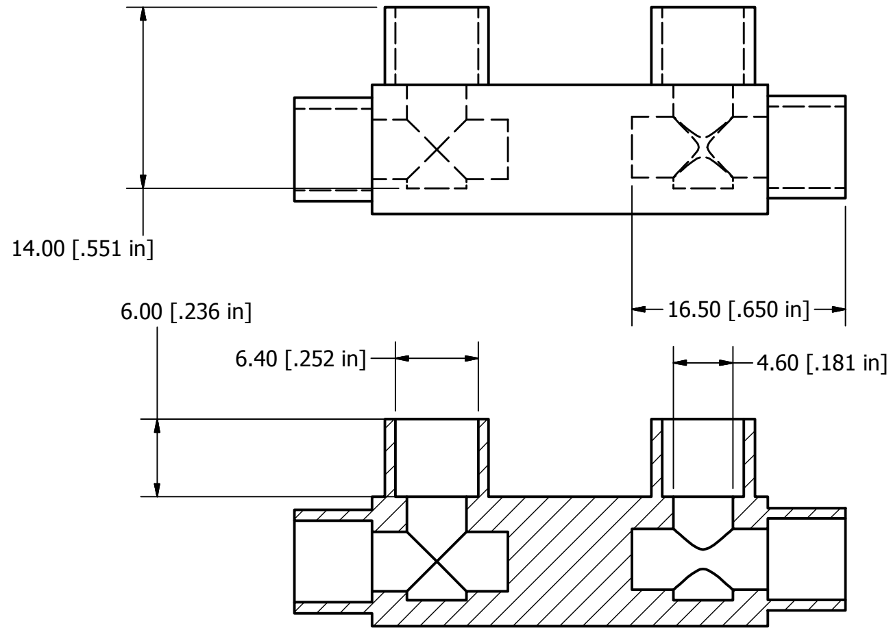
SECTION A-A SCALE 2.5
